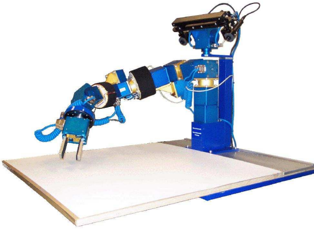
Fig. 1. The anthropomorphic robotic assistant CORA.
