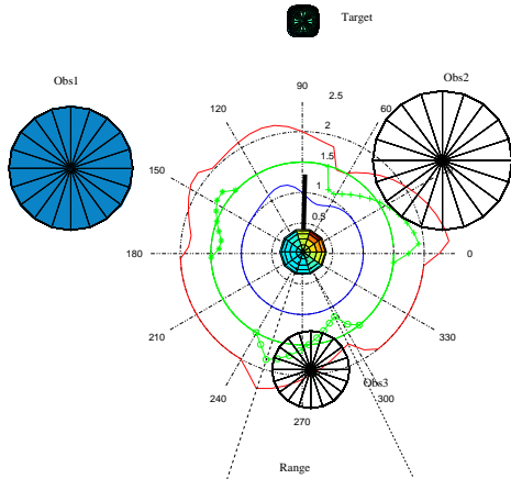
Fig. 6. Target acquisition and obstacle avoidance. Depicted is the phaseplot of the dynamical system concerning the contribution of three obstacles and one target in polar coordinates with \dot{\phi} = r(\phi) . The target is specifying an attractor (negative slope) and obstacles are specifying repellers.
